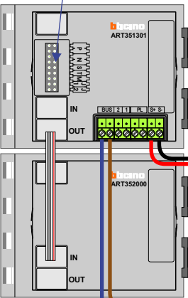
DEURSTATION S-151V
