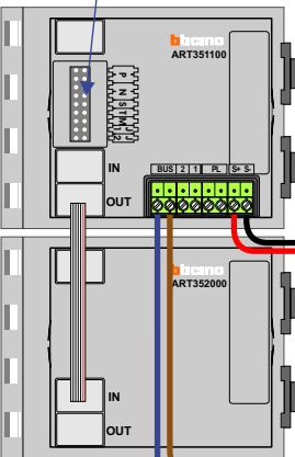
DEURSTATION S-151A
