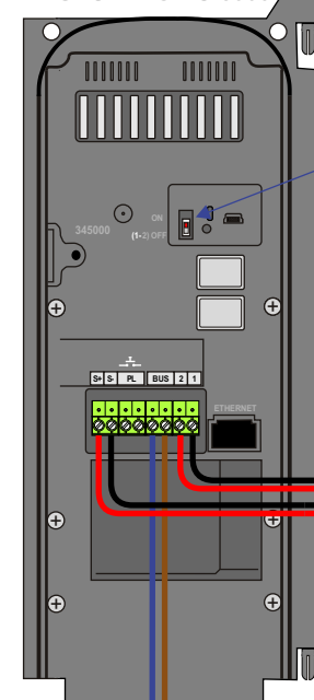
DEURSTATION S-5000
